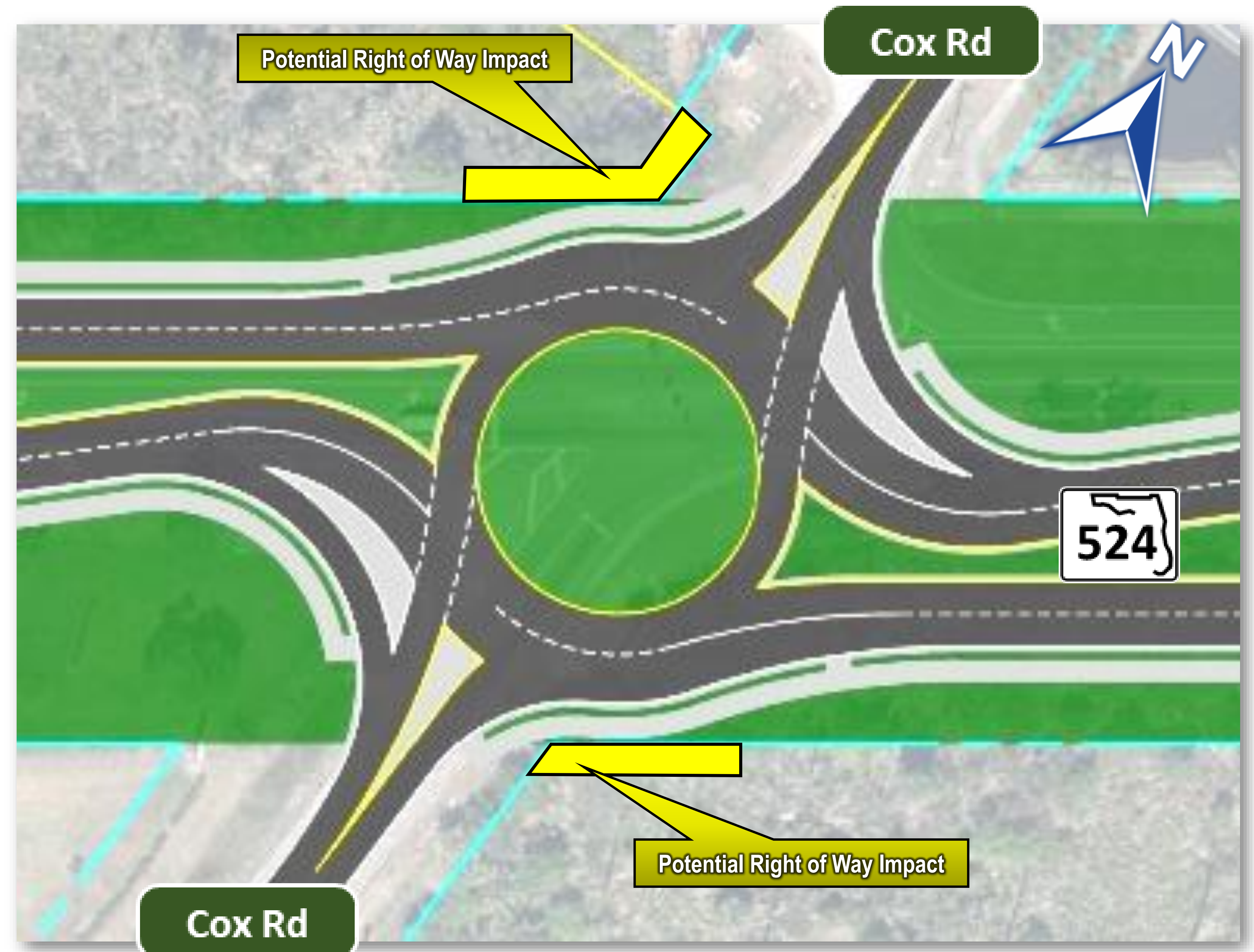
Roundabout Alternative
