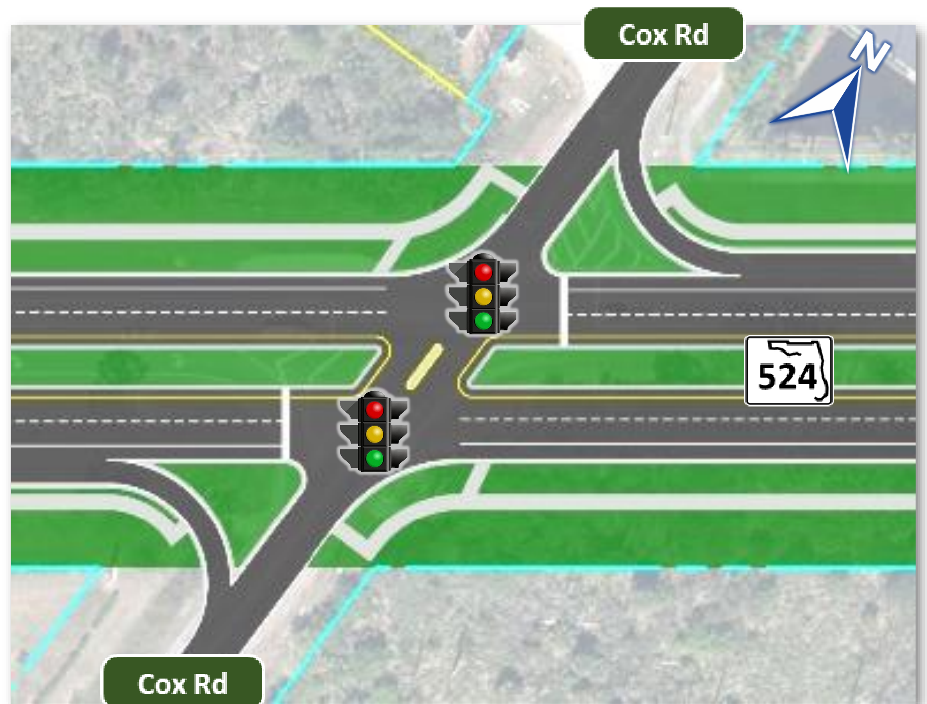
Median U-Turn (MUT) Alternative
