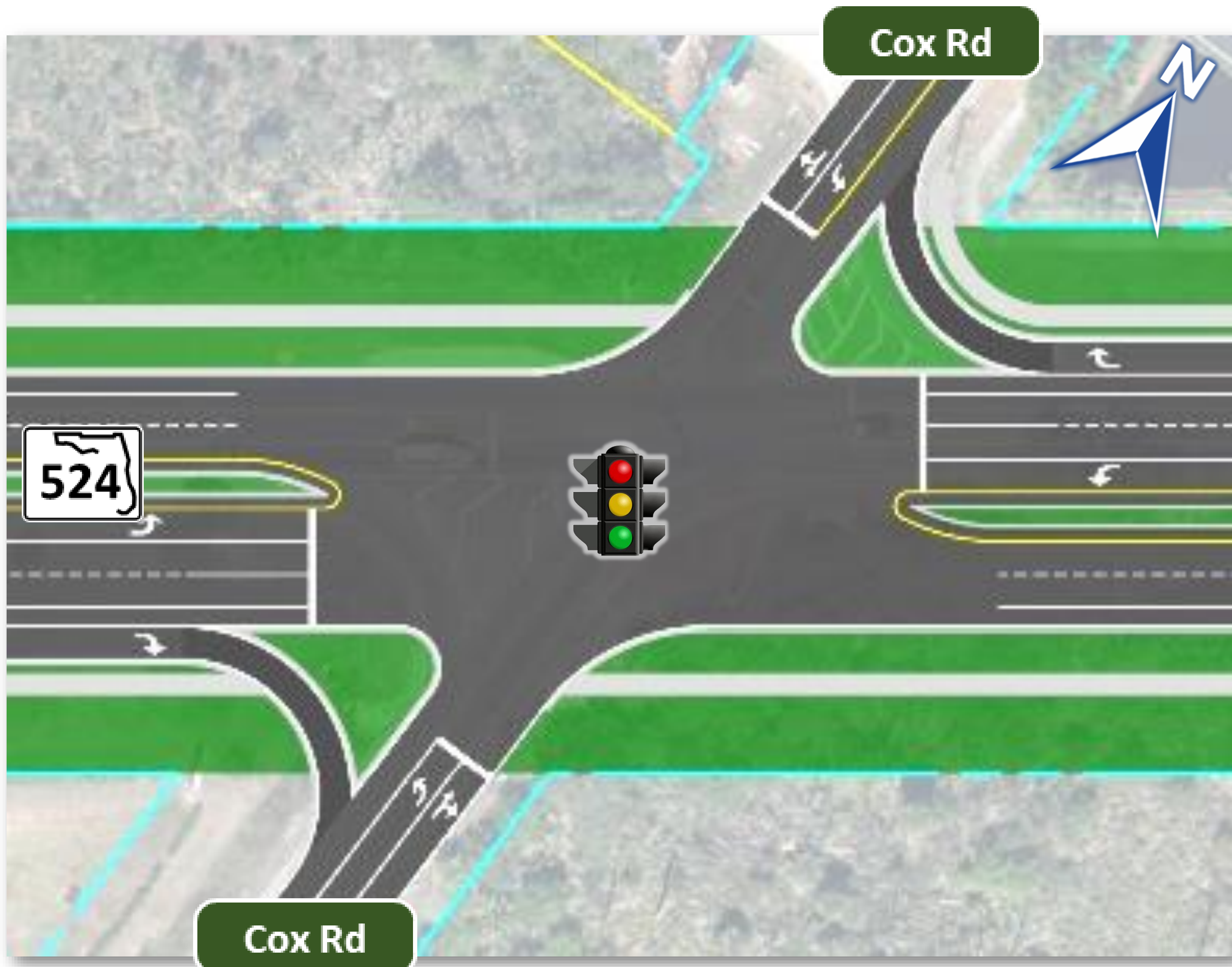
Signalized Alternative
