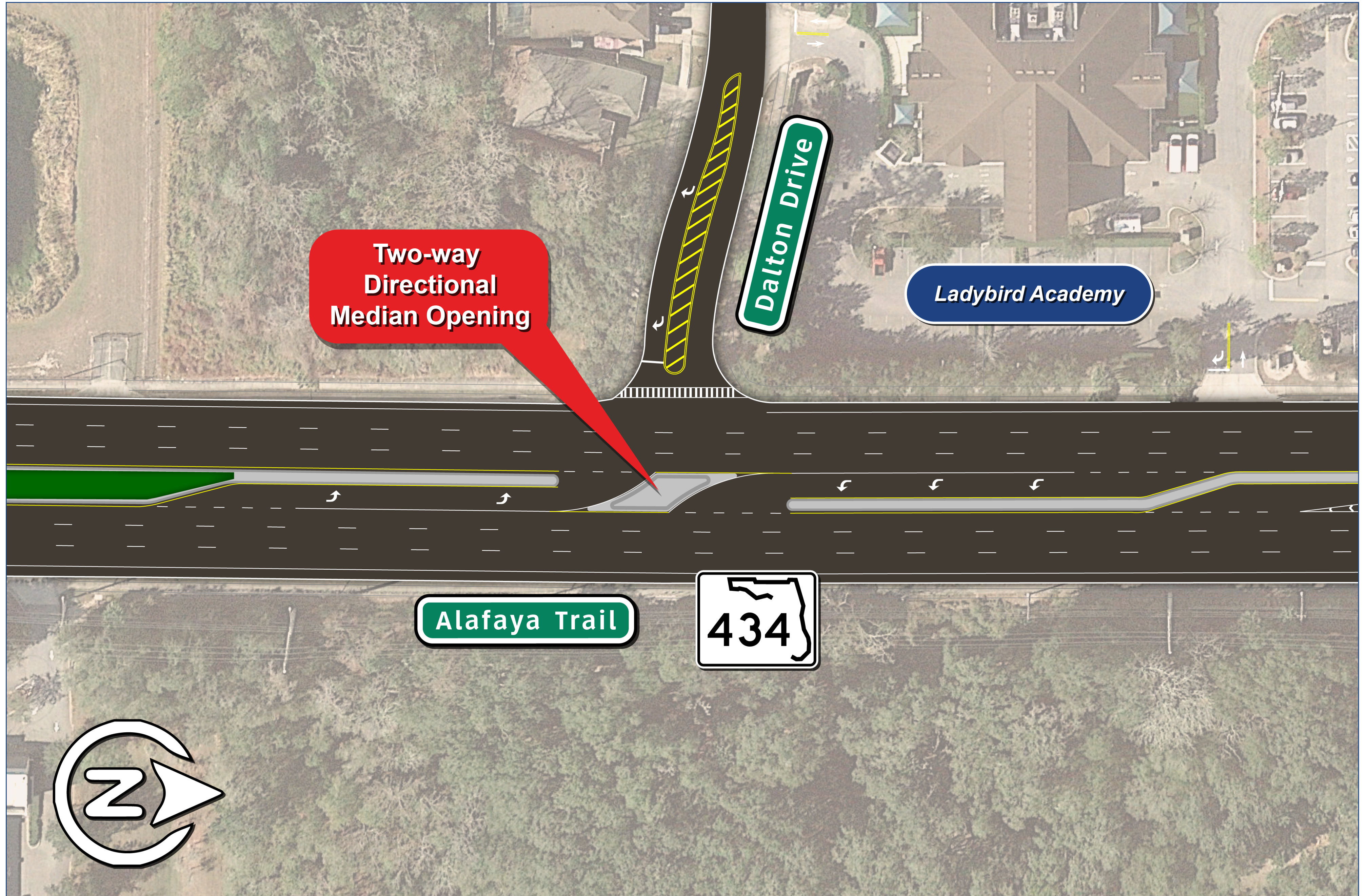
Alafaya Trail (S.R. 434) at Dalton Drive
