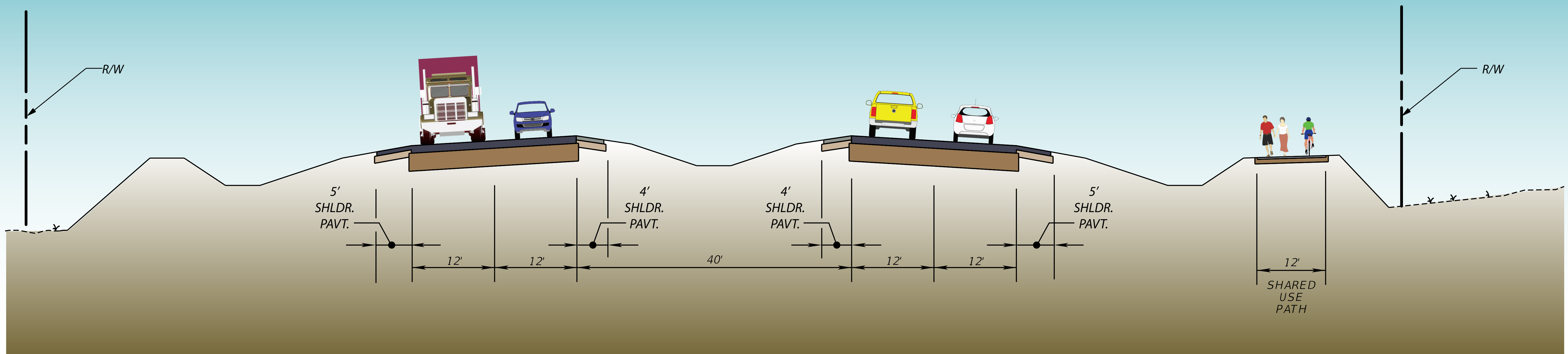
TYPICAL SECTION No. 2 FROM THE WITHLACOOCHEE STATE FOREST TO EAST OF CR 478A
