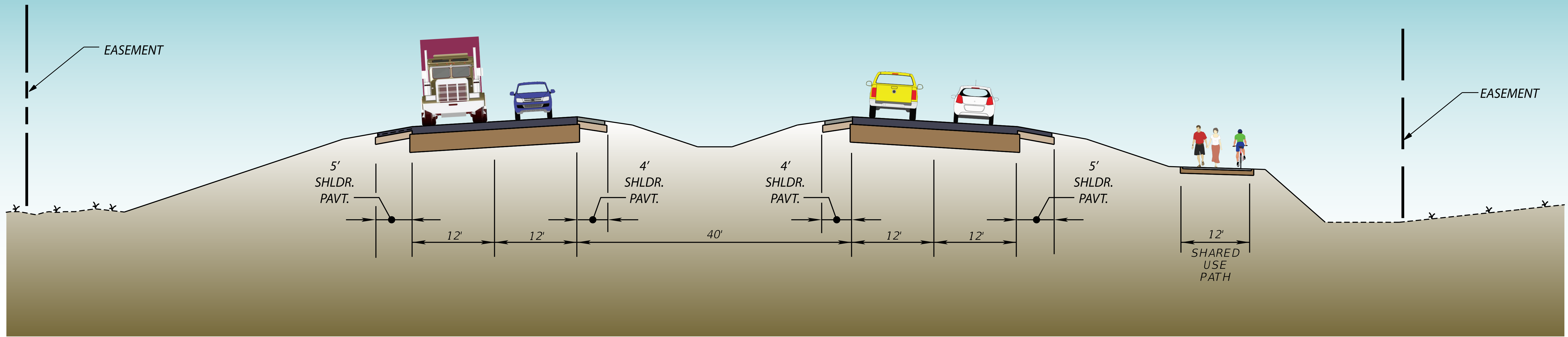
TYPICAL SECTION No. 1 FROM THE COUNTY LINE TO THE LIMITS OF THE WITHLACOOCHEE STATE FOREST
