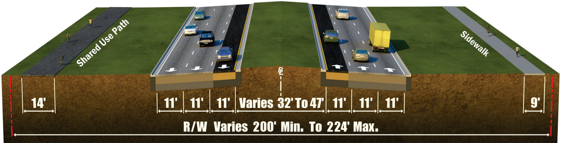
Inside Widening with Shared Use Path Posted Speed Limit: 45 mph
