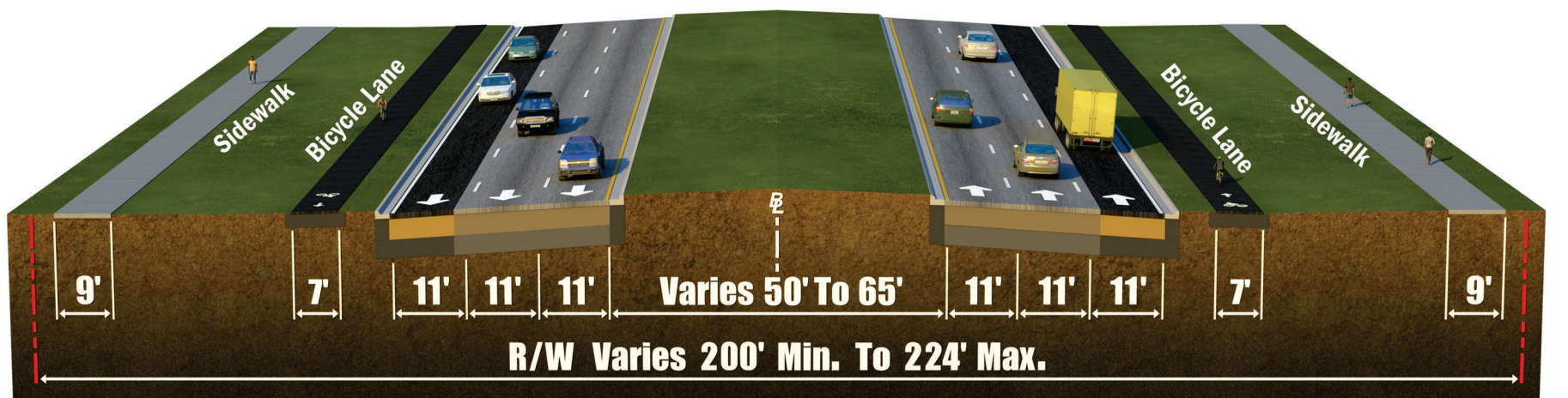
Outside Widening with Separated Bicycle Lanes Posted Speed Limit: 45 mph
