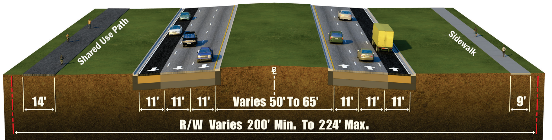
Outside Widening with Shared Use Path Posted Speed Limit: 45 mph
