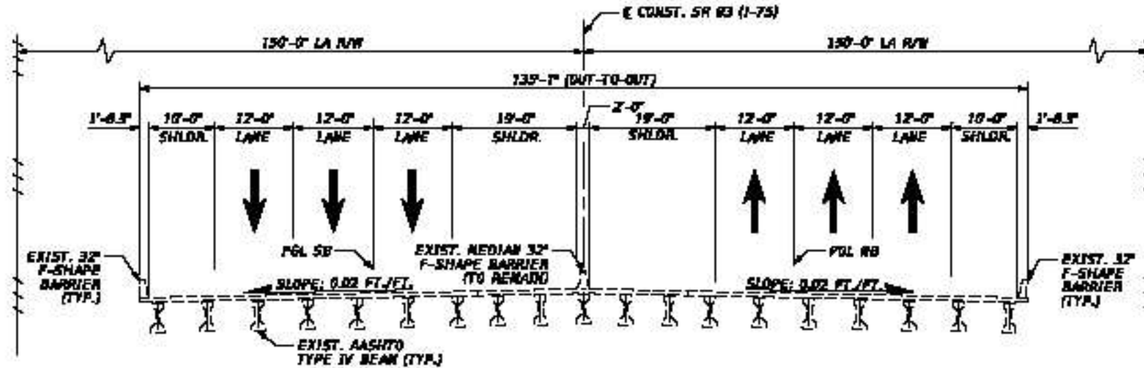
EXISTING SECTION THROUGH BRIDGE DECK
