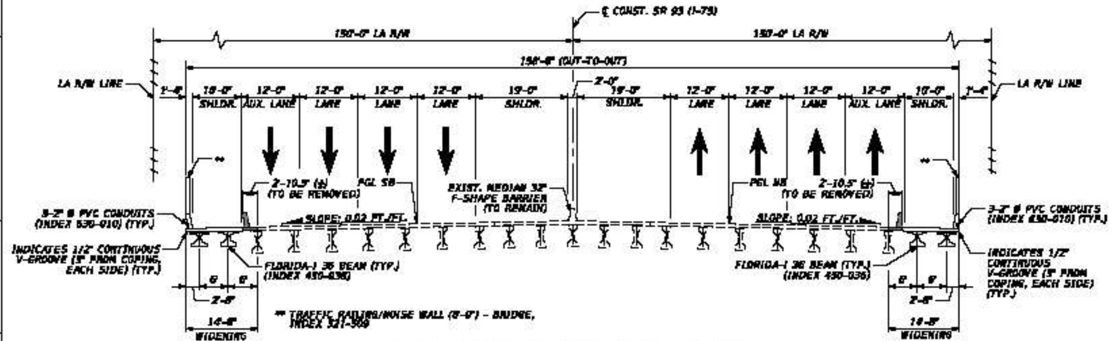
PROPOSED SECTION THROUGH BRIDGE DECK
