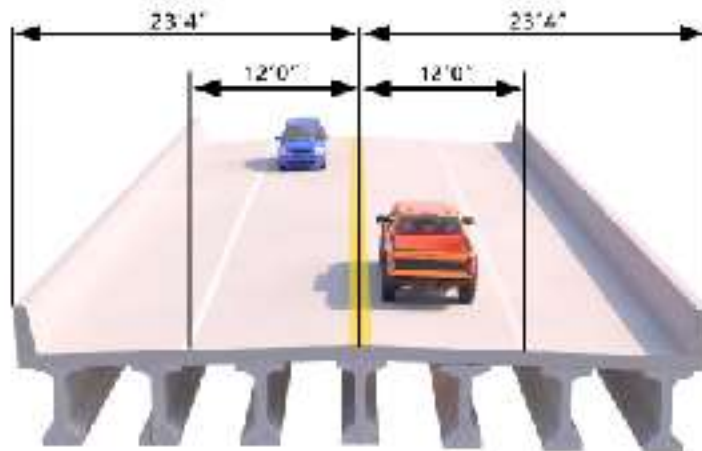
Figure 7-2 | Bridge 360049 Typical Section
