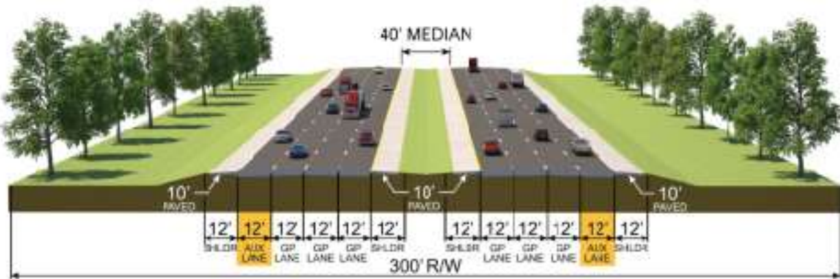
Figure 5-1 | Build Alternative Typical Section
