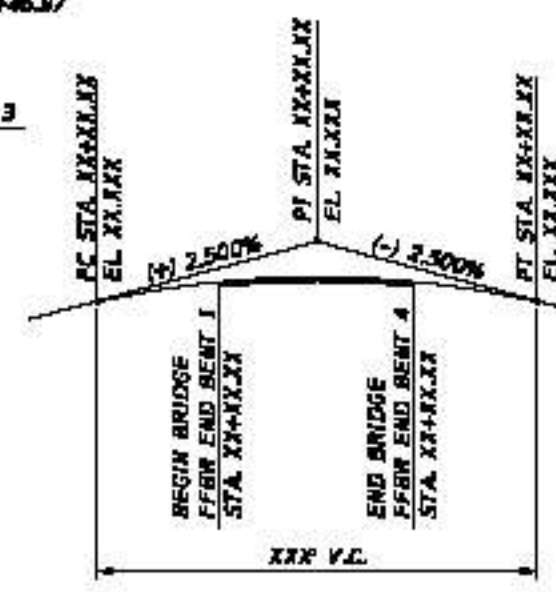
VERTICAL CURVE DATA
