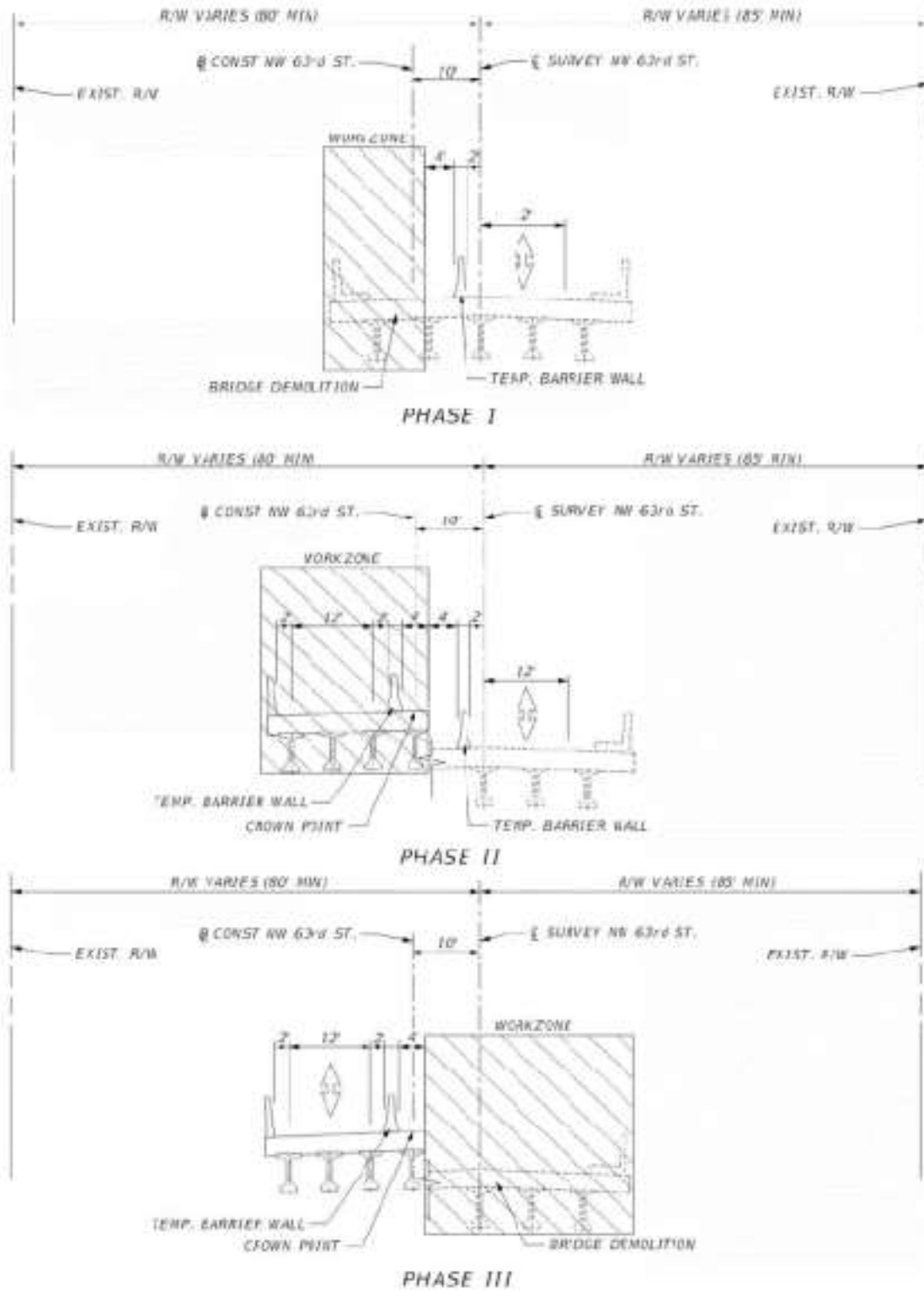
Figure 7-4 | SW 63 rd Street Construction Phasing
