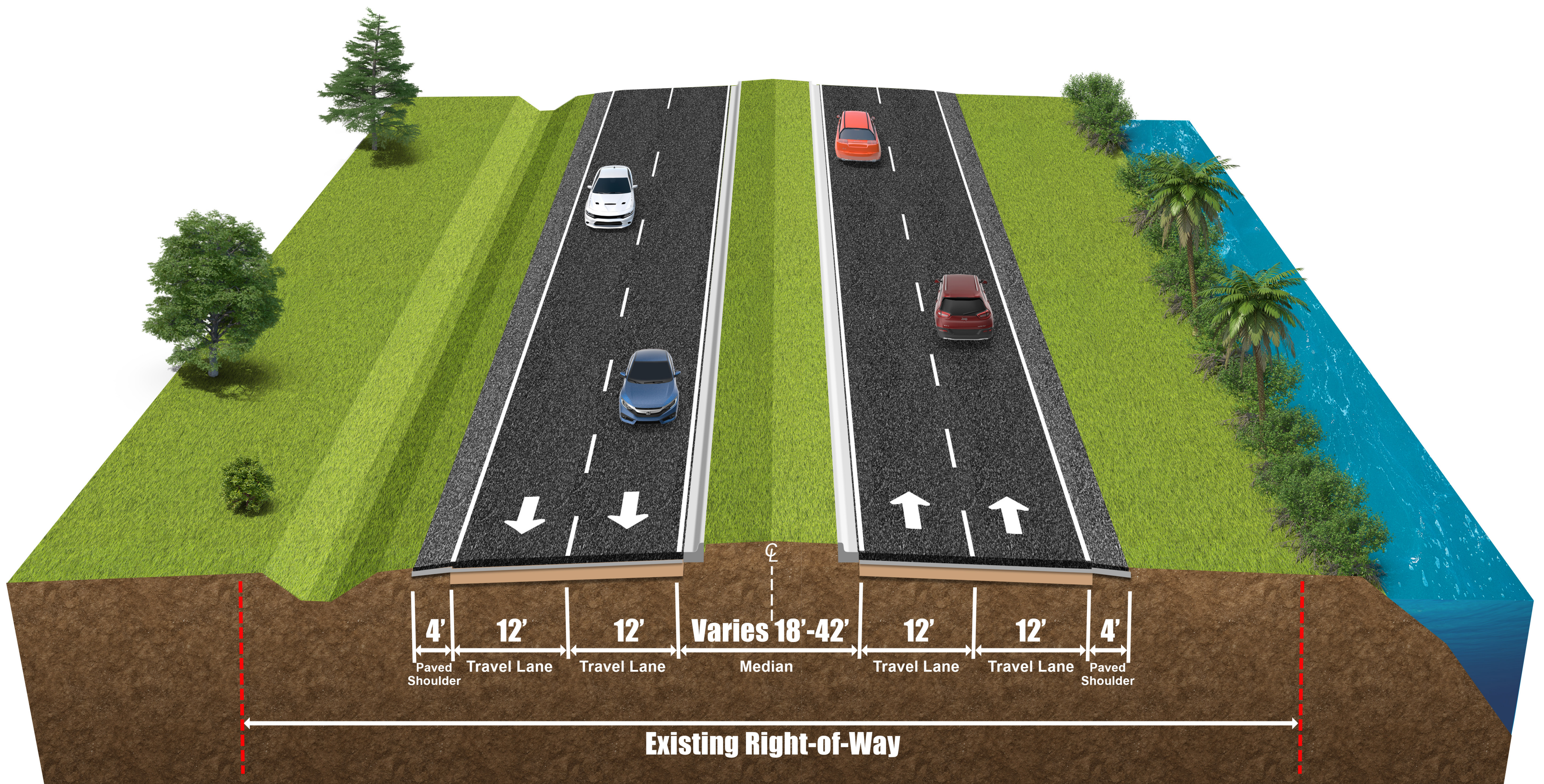
State Road 5 (US 1) Existing Typical Section
