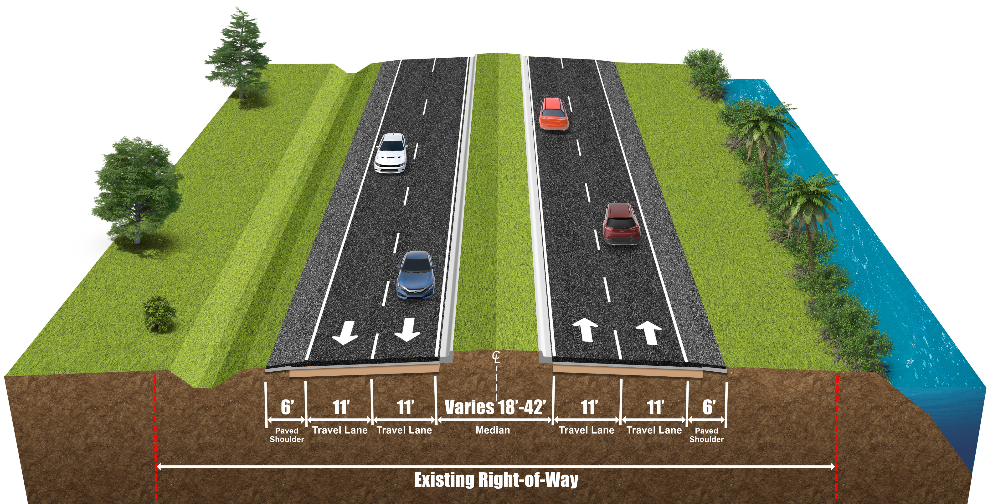
State Road 5 (US 1) Proposed Typical Section
