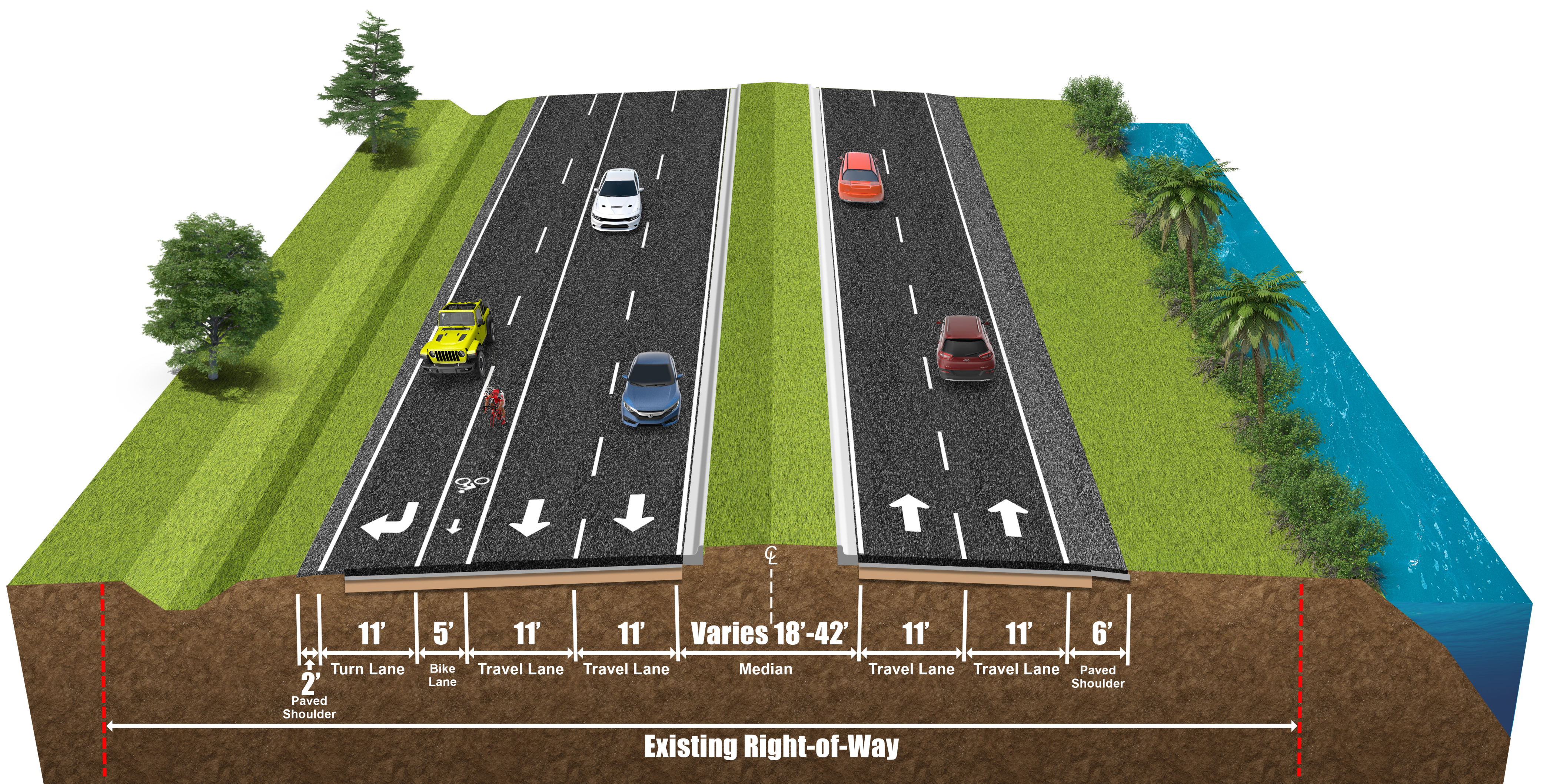
State Road 5 (US 1) Proposed Turn Lane and Bicycle Keyhole Typical Section
