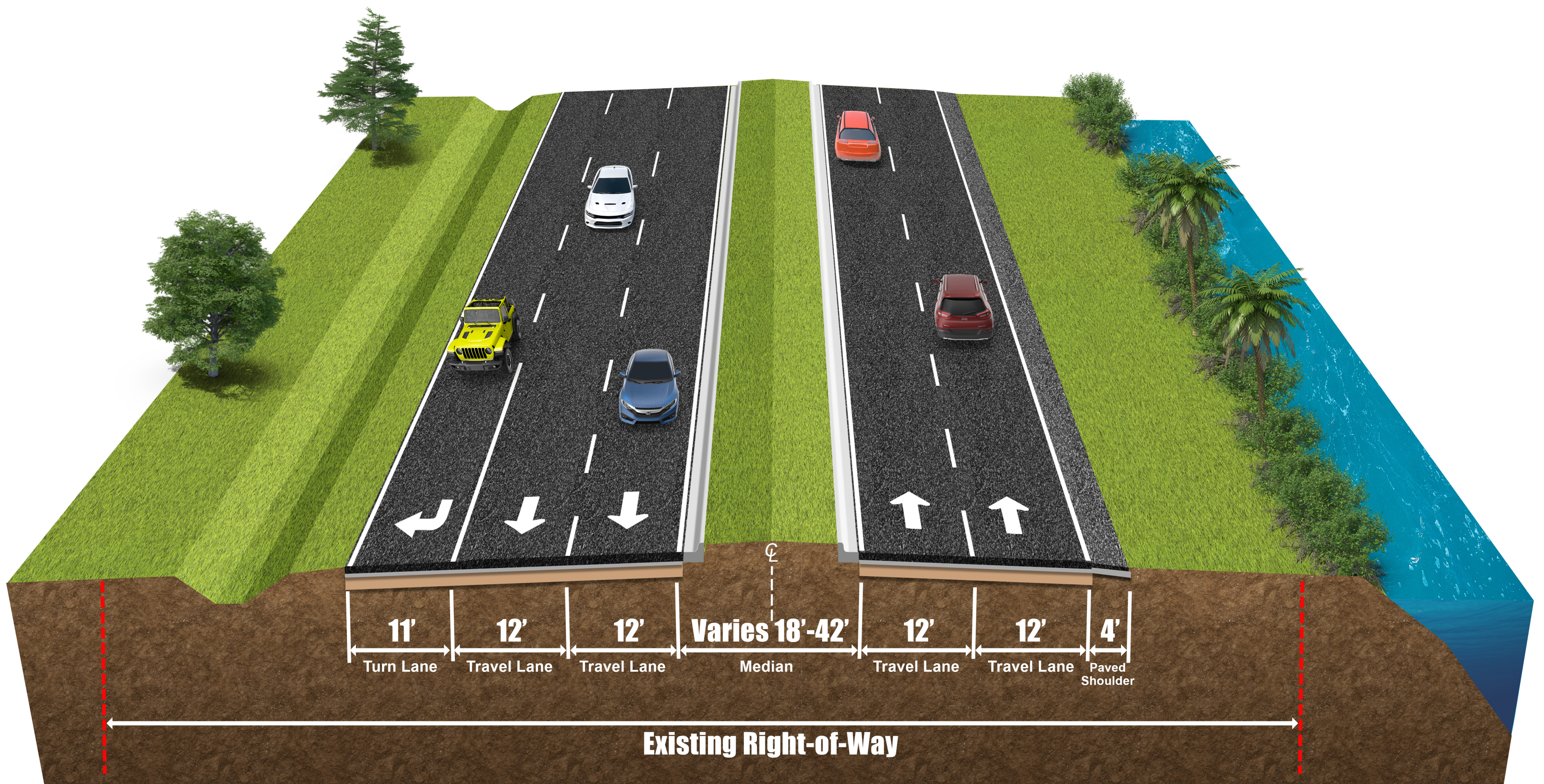
State Road 5 (US 1) Existing Turn Lane Typical Section
