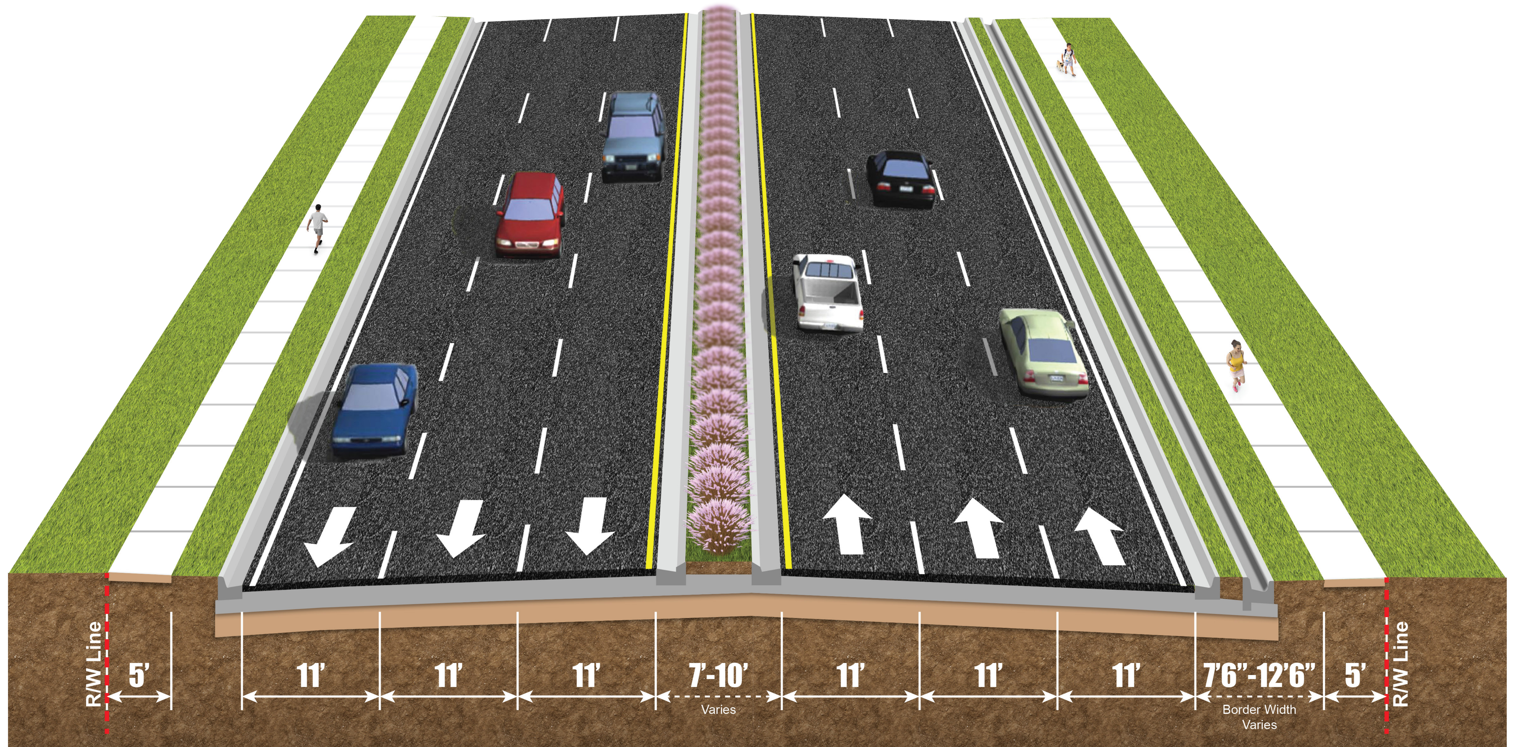
Typical Section of Raised Landscaped Median East of I-75 to SW 20th Avenue & SW 16th Avenue to S. Pine Avenue
